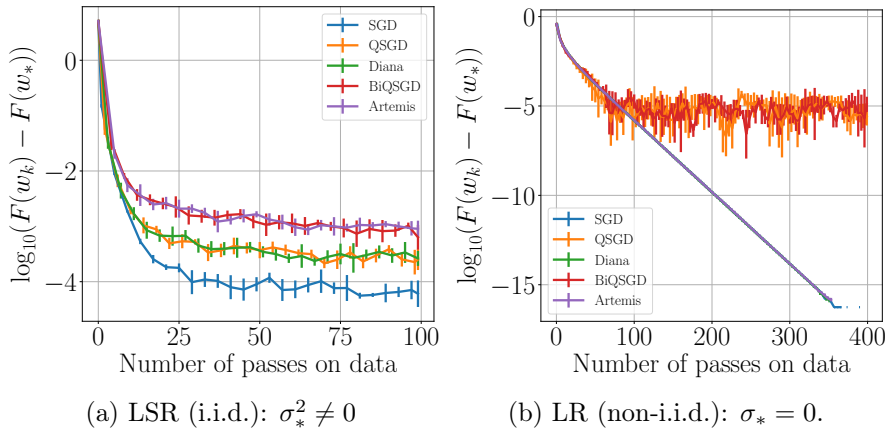
Figure 2.1: Left: illustration of the saturation when \sigma_* \neq 0 and data is i.i.d., right: illustration of the memory benefits when \sigma_* = 0 but with non-i.i.d. data.
