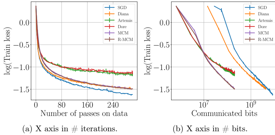
Figure C.9: Convergence on MNIST using a CNN.
