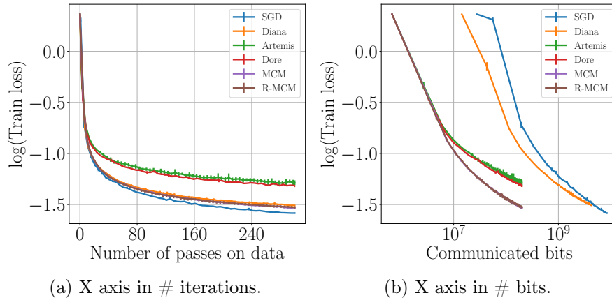
Figure C.11: Convergence on FE-MNIST.
