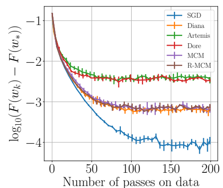
Figure 1.10: MCM and Rand-MCM on quantum, they achieves a rate of convergence identical to unidirectional compression.
