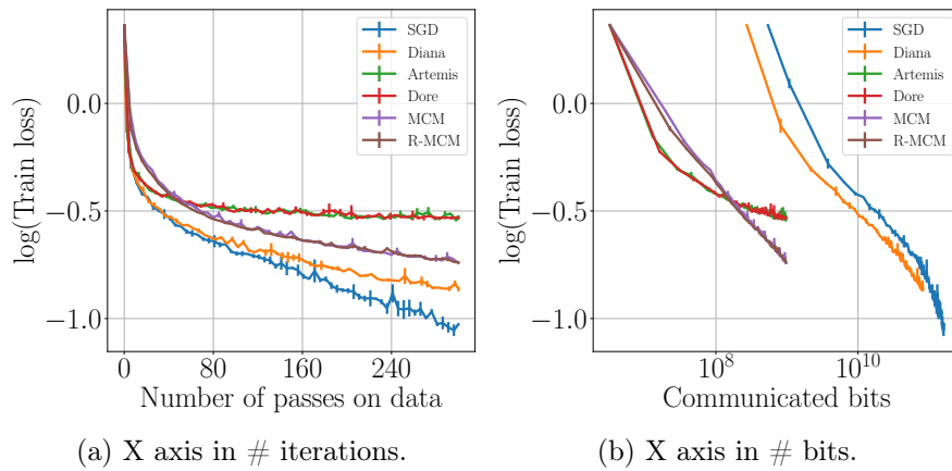
Figure C.10: Convergence on Fashion-MNIST.
