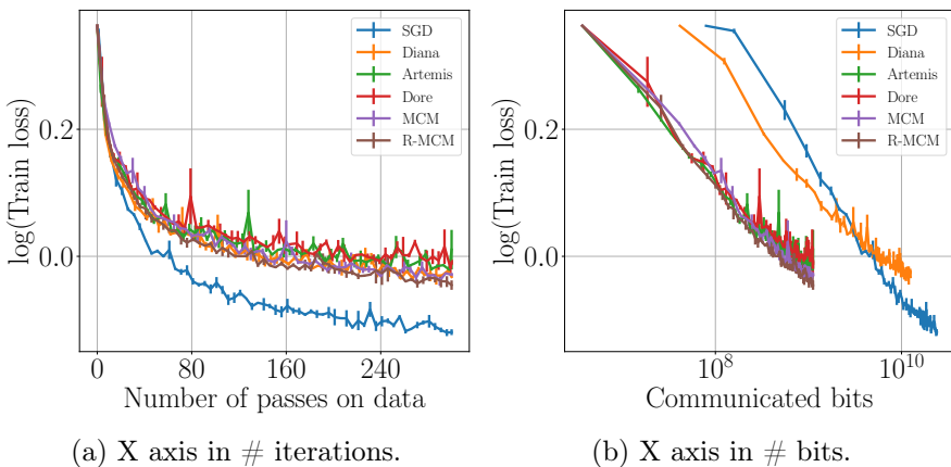
Figure C.12: Convergence on CIFAR10.
